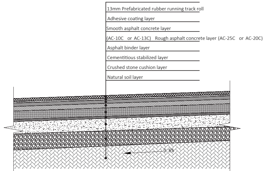
Runway foundation section diagram
